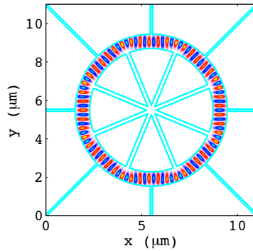
Figure 1. Circular wiggler resonator with wiggler mode simulated using 2D eigenmode solver.
