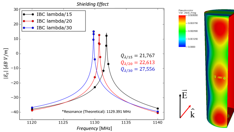
Figure 1: (a) Shielding Effectiveness (b) Surface Current Distribution.
