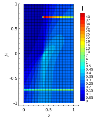
Fig. 3. Scattering from a point source in a Rayleigh scattering medium.
