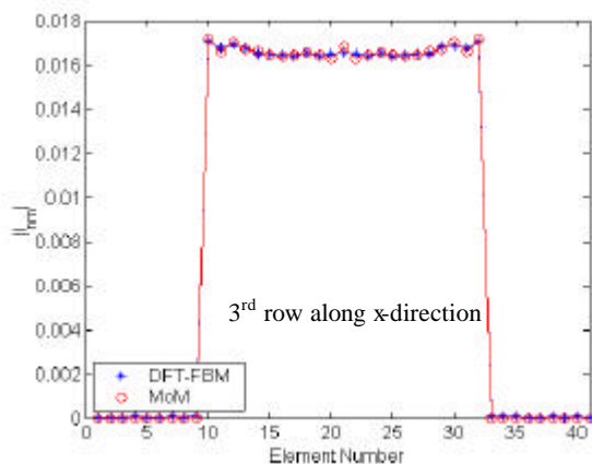
Fig.2 Comparison of current distributions obtained by MoM and DFT-FBM on 749 element elliptical printed dipole array ; d_x = d_y = 0.5 l_0 , length of dipole = 0.3 l_0 , width of dipole = 0.01 l_0 , \epsilon_r = 2.55 , substrate thickness = 0.06 l_0
