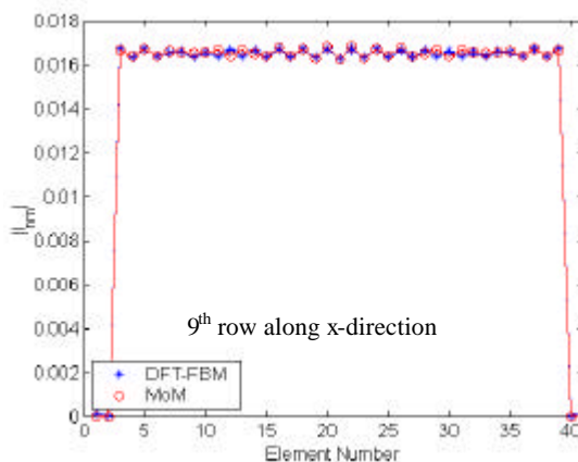
Fig.2 Comparison of current distributions obtained by MoM and DFT-FBM on 749 element elliptical printed dipole array ; d_x = d_y = 0.5 l_0 , length of dipole = 0.3 l_0 , width of dipole = 0.01 l_0 , \epsilon_r = 2.55 , substrate thickness = 0.06 l_0
