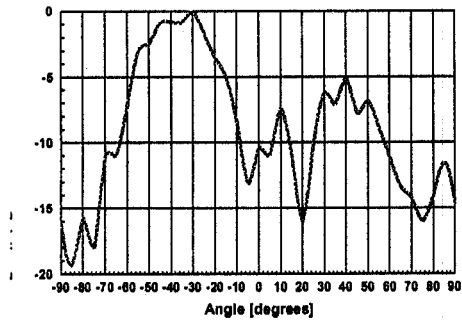
Fig. 11. Measured bistatic RCS (frequency : 5.2 GHz, -30°).
