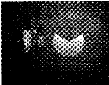
Fig. 1. AlGaIn/GaN HEMT AIA power amplifier.
