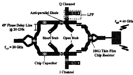
Fig. 6. Modulator/demodulator integrated with a planar antenna.
