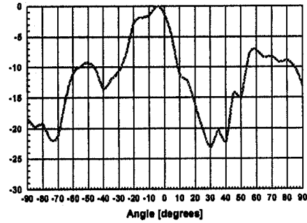
Fig. 12. Measured bistatic RCS (frequency : 5.8 GHz, 0°).
