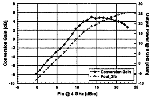
Fig. 5. Output power and conversion gain versus input power.
