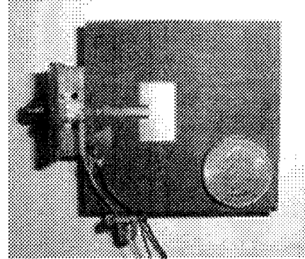
Fig. 4. AIA AlGaIn/GaN HEMT frequency doubler.
