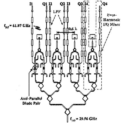
Fig. 8. 60 GHz four-element integrated phased array with I/Q mixers (Circuit size : 13.3 x 20 mm).
