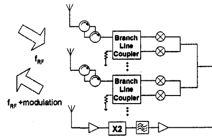
Fig. 10. Schematic of frequency autonomous retrodirective array.
