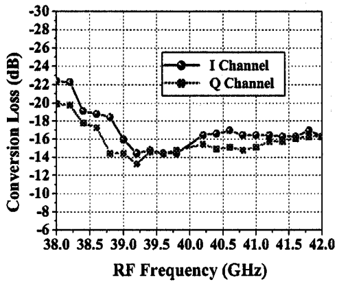
Fig. 7. Conversion loss with respect to RF frequency for each I and Q channel (LO : 11.8 dBm).
