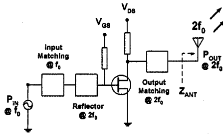
Fig. 3. Frequency doubler using AIA design approach.
