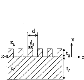
Fig. 1: Dielectric grating structure.
