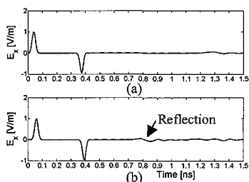
Fig. 2. Antenna Response for Tissue Samples: (a) Healthy (b) Diseased, via 1D FDTD
