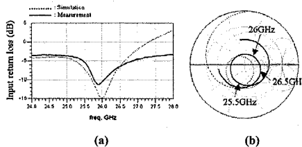
Figure 2: Input return loss (S11 in dB) (a), input impedance loci (b)
