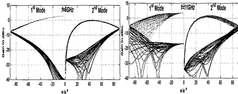
Figure. Dual-mode radiation patterns at 6GHz and 11GHz.
