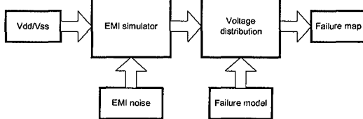
Fig. 3. EMI simulator and Failure map.
