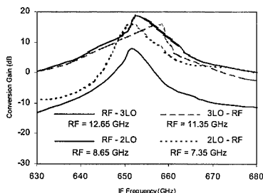
Fig. 2. Conversion gain versus IF frequency of RF frequency centered at 12.65, 11.35, 8.65 and 7.35 GHz
