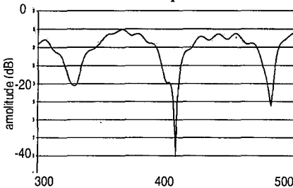
Fig 1 Reflection Coeff of TWA vs. f (MHz) for R = 499
