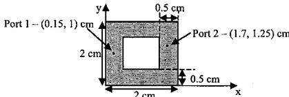
Fig. 1. Rectangular Ring Plane for Comparison with HFSS
