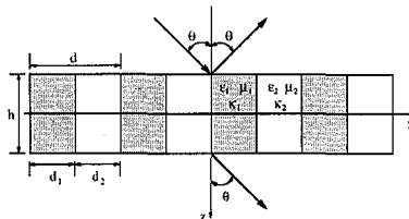
Fig. 1. Configuration of a chiral grating.
