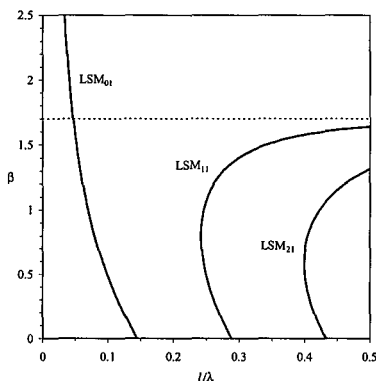
Fig. 2 Dispersion diagram
