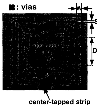
Figure1. Top view of a symmetrical on-chip transformer fabricated using silicon IC technology.
