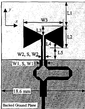
Fig. 1. Antenna geometry.
