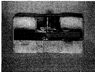
Figure 1: The prototype folded-dipole antenna with an integrated symmetrizing device. Behind the antenna a foam layer and the mushroom surface are seen.
