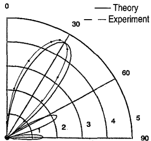
Fig 2 Elevation Pattern of TWA
