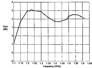
Figure 2: Measured Gain (dB)
