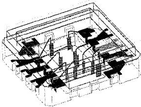
Fig. 1. Model the bonding wires together in the package to consider the mutual coupling among the bonding wires, package and die pattern.
