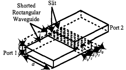
Fig.1 Conventional phase shifter
