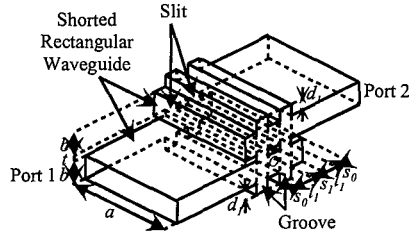
Fig.2 Phase shifter with grooves
