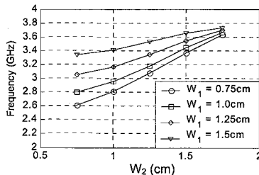
Fig. 4. Design graph for choosing dimensions of L-Shaped plane
