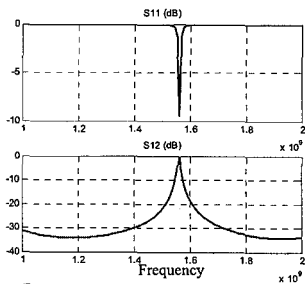
Fig 2a: S_{11} (dB) and S_{12} (dB)
