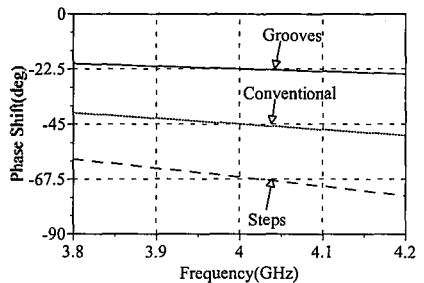
Fig.4 Transmission phase
