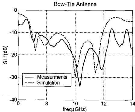
Fig. 2. Measured and simulated return loss.
