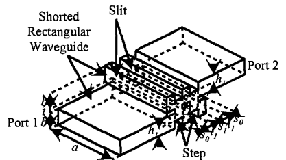
Fig.3 Phase shifter with steps
