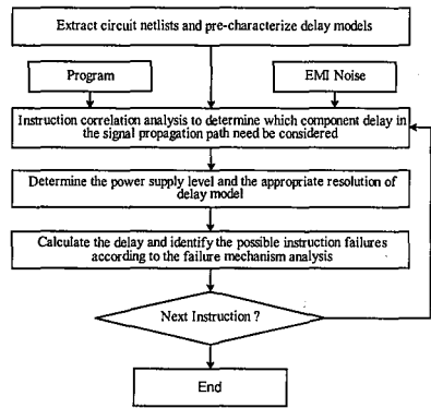
Fig. 2. EMI noise induced instruction failure simulation procedure
