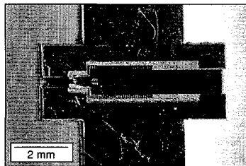
Fig. 2. Membrane supported frequency tripler integrated with waveguide transition.
