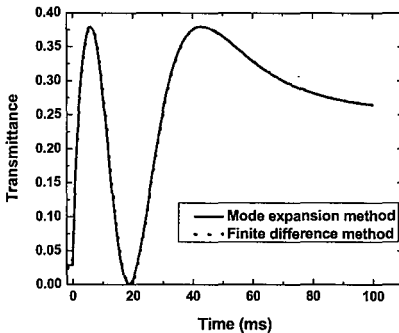
Fig. 1. Electro-optic curve of a PA E-7 cell at d = 4.04 \mu\text{m} , \lambda = 632.8 \text{nm} , T = 22^\circ after released from 10Vrms. The solid line is for mode expansion method, while the dot line is for finite difference method.
