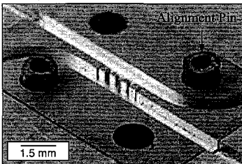
Fig. 1. Micromachined branch-guide coupler with high definition structures.
