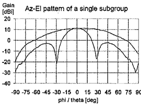
Fig. 3: Farfield Pattern of a Single Subgroup
