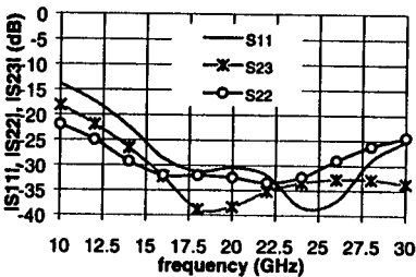
Figure 1: HFSS Simulation.
