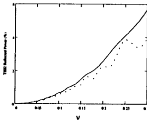
Fig. 2: Reflected power in the TE_{02} mode vs slope of the transition. Comparison between the theoretical values (solid line) and the Mode Matching and GSM results (dotted line).
