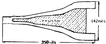
Figure 2: The power divider.
