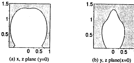
Fig. 1 Typical Shape of Readzone for a Vertically Polarized Dipole Tag. ( Units are in meters )
