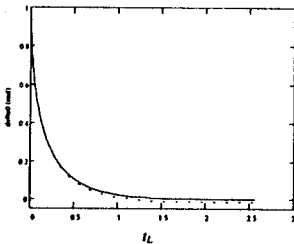
Fig. 1: \delta_0 (parameter that gives the dependence of the phase of the reflection coefficient) vs t_L (parameter related with the length of the transition). Comparison between the theoretical values (solid line) and the Mode Matching and GSM results (dotted line).
