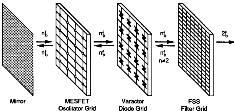
Figure 1: Configuration of the Free-Space Frequency Filtered System.
