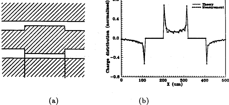
Figure 1. A step in impedance CPW test structure (a) and the theoretical and measured charge distribution on a transverse cross section (b).
