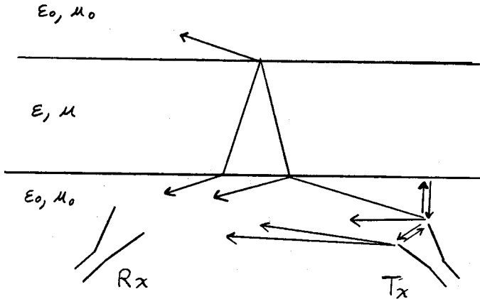
Figure: A few of the many possible coupling paths
